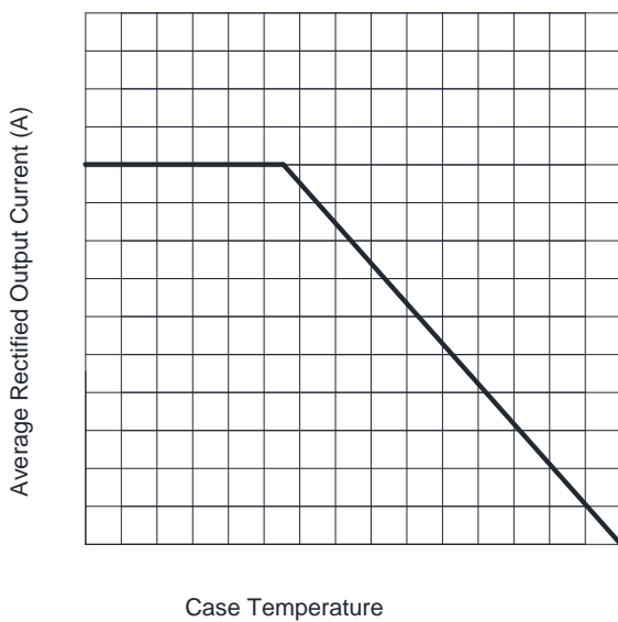
FIG1:Io-Tc Curve
